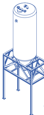
Silos with unloading on truck
